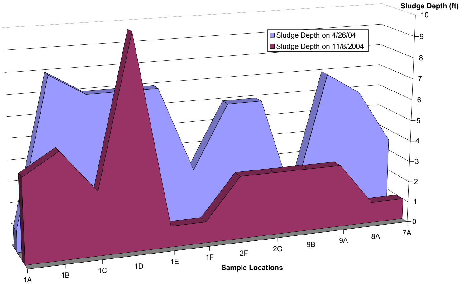
Sludge Blanket Profile from a City in Indiana Wastewater Lagoon System Before and After Using BIO ENERGIZER
